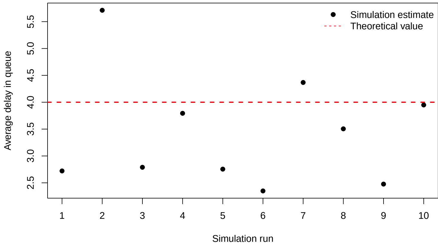
M/M/1 average queue delay across 10 runs
